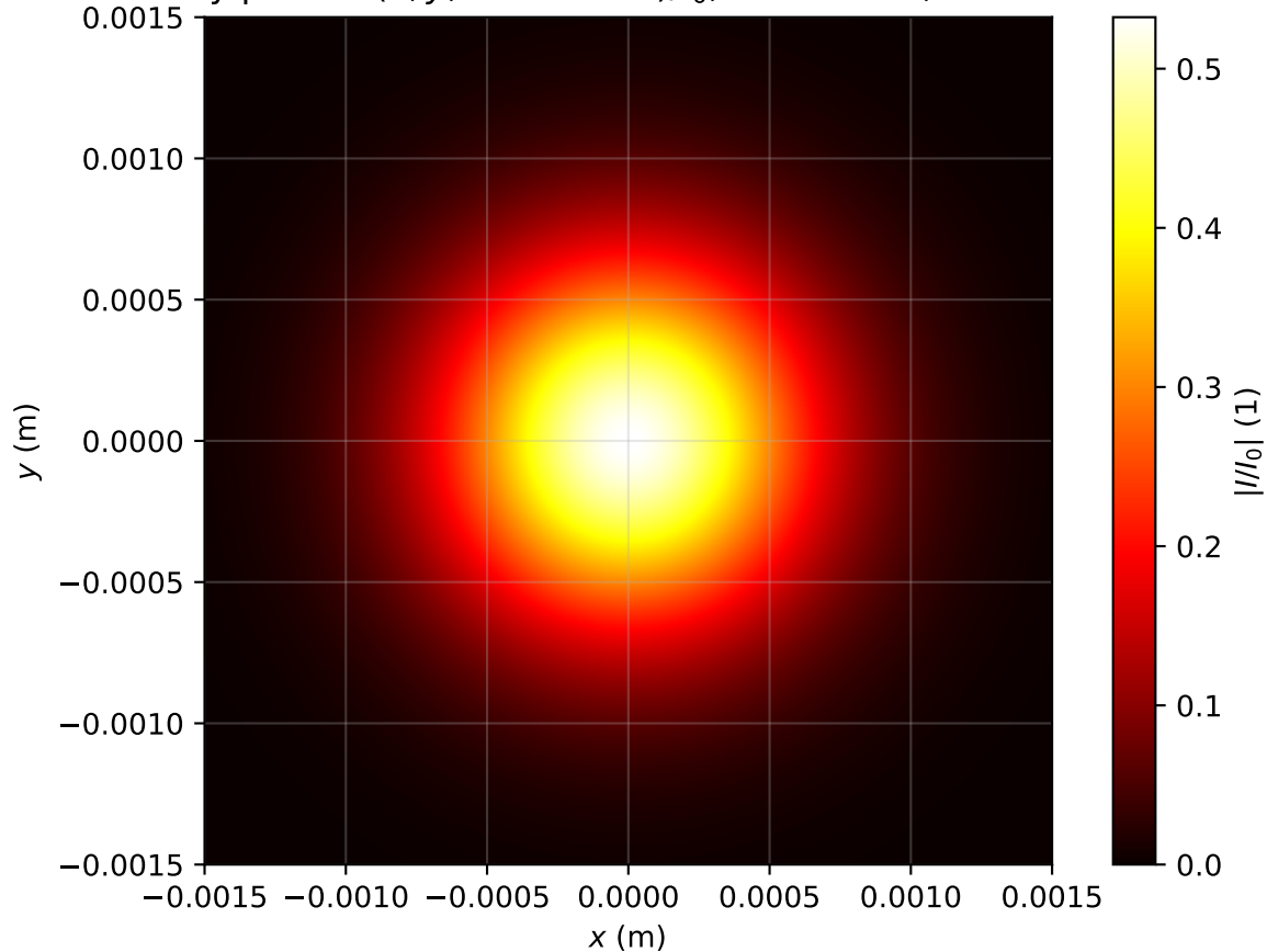
Intensity profile I(x, y, z = 2.229m)/I_0 , Pin=0.2Pcr, artificial time
